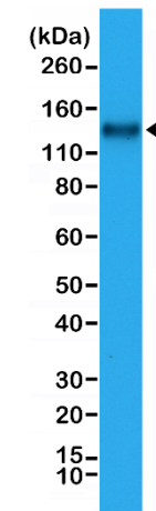
Western Blot of Jurkat cell lysate, using Anti-CD31 RM247 at a 1:1000 dilution, showed CD31 (~130 kDa) expression in Jurkat cells.
