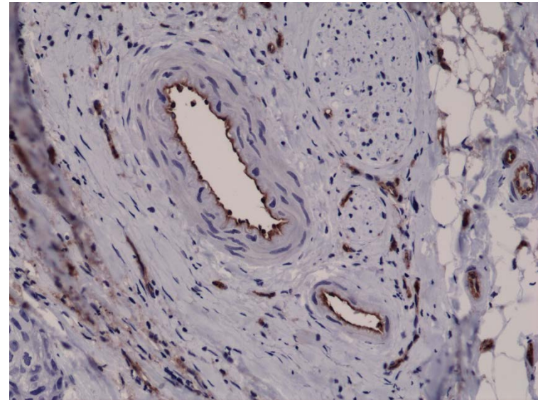
Immunohistochemical staining of formalin fixed and paraffin embedded human breast cancer tissue sections using Anti-CD31 RM247 at a 1:2500 dilution.
